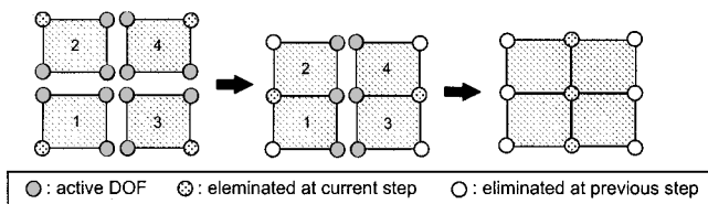
Fig. 2 Elimination process of the multifrontal method.
