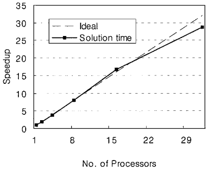
Fig. 9 Speedup for 32 × 32 × 16 solid elements.
