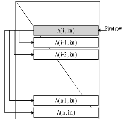
Fig. 6 Gauss-elimination using i th row as pivot.
