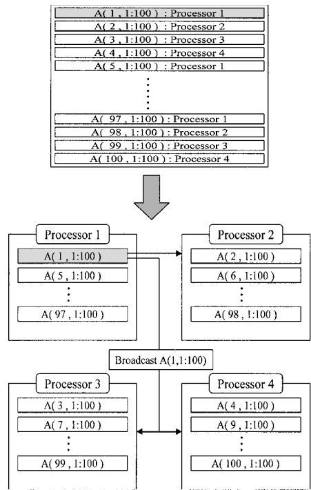
Fig. 7 Distribution of matrix for parallel Gauss elimination.
