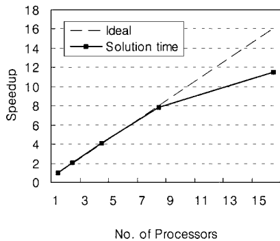
Fig. 8 Speedup for 16 × 16 × 16 solid elements.
